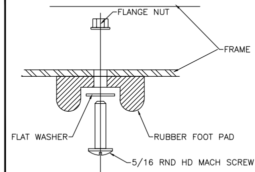
④ RUBBER FOOT PAD ATTACH. DETAIL
