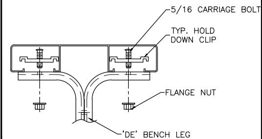
② TYP 2x10 ENDCAP ATTACHMENT
