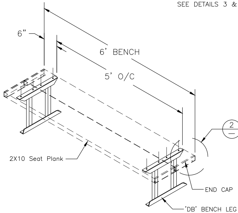
ISOMETRIC VIEW OF BENCH ASSEMBLY
