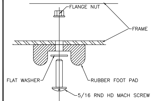
RUBBER FOOT PAD ATTACH. DETAIL
