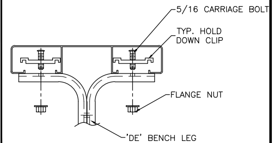
TYP 2x10 ENDCAP ATTACHMENT
