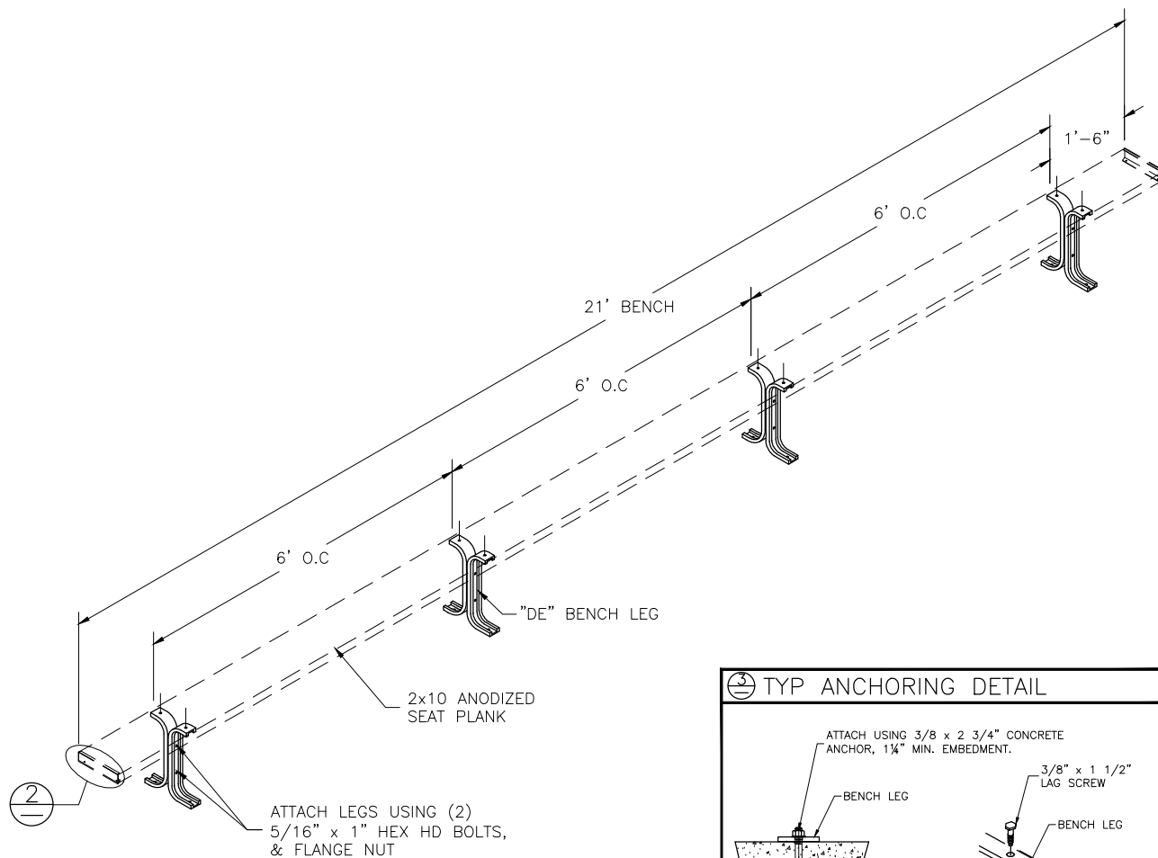
ISOMETRIC OF BENCH ASSEMBLY
