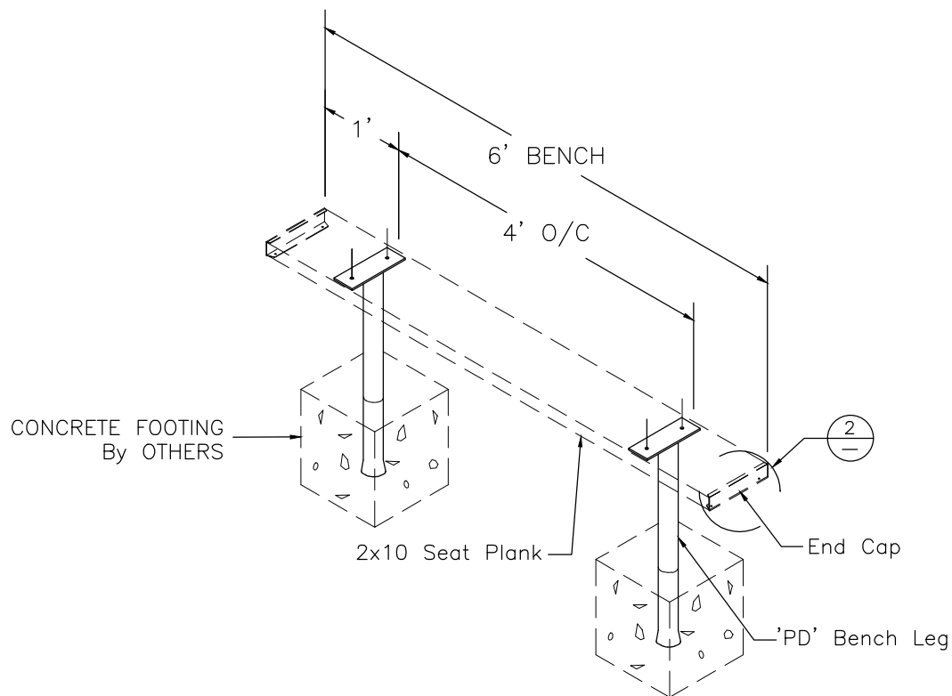
ISOMETRIC VIEW OF BENCH ASSEMBLY
