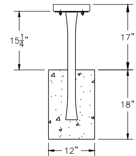
PERMANENT BENCH HEIGHT DETAIL
