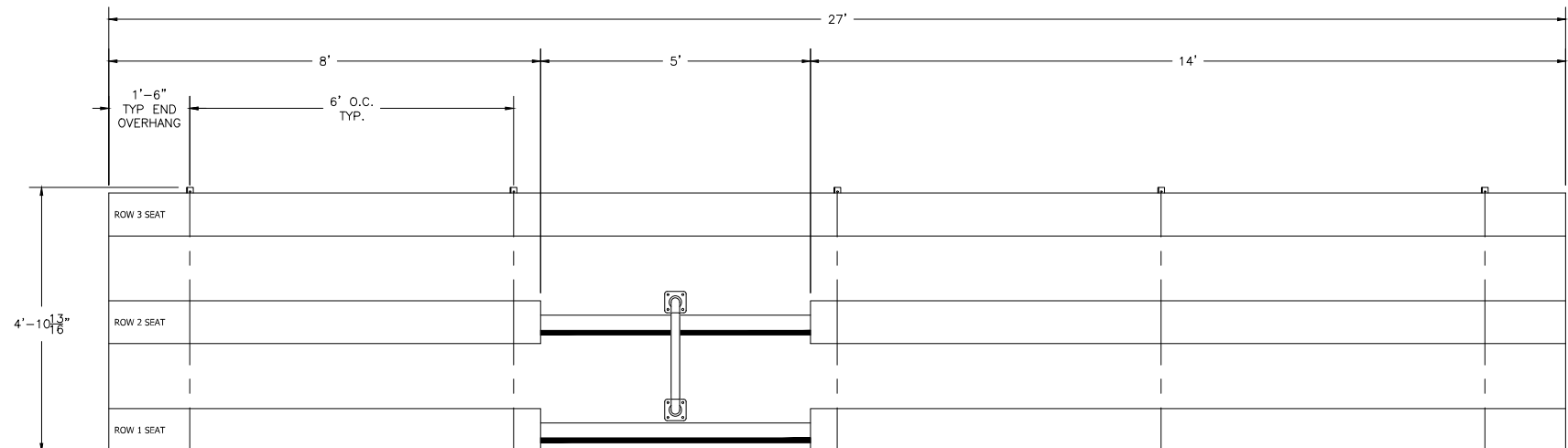
BLEACHER TOP VIEW
